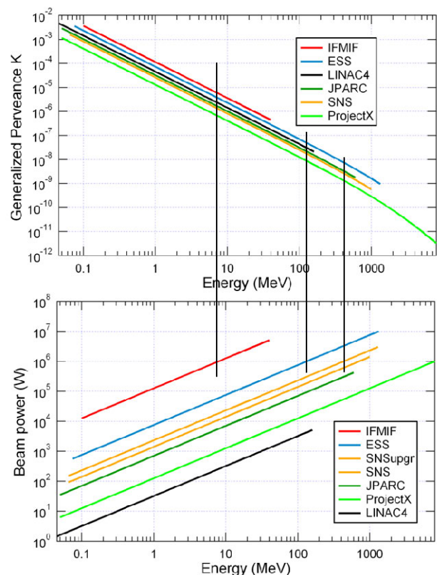
Figure 1 and 2: Generalise perveance K and beam power as functions of energy 2.
