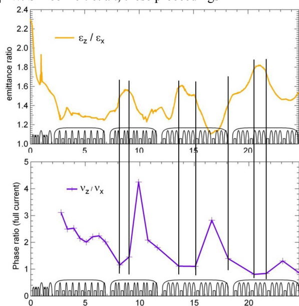
Figure 5: Variation of emittance ratio and tune ratio along the MEBT and the 4 cryomodules of the SRF-Linac
