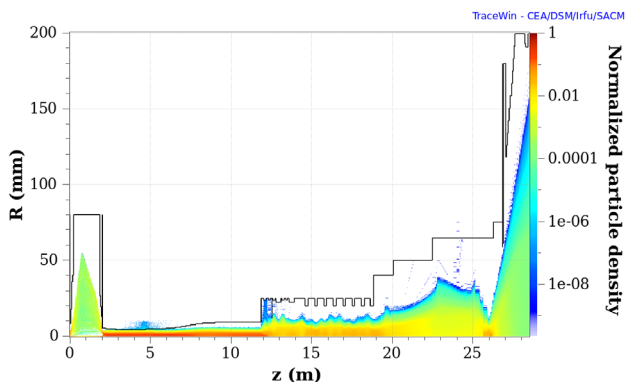
Figure 2: Beam density along the IFMIF/EVEDA prototype accelerator. Simulation performed with 10^7 particles.
