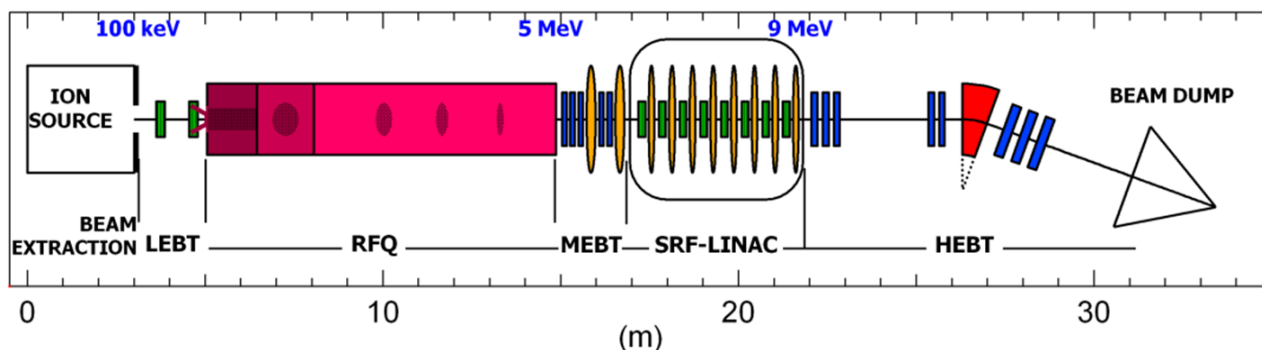
Figure 1: Scheme of the IFMIF-EVEDA prototype accelerator.
