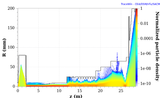
Figure 3: Cumulated densities for 150 runs (with errors), with 1.1 \times 10^6 particles each.
