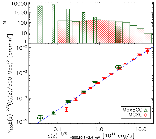
Fig. 11. Bottom panel: Comparison between our results (red diamonds, as in left-hand panel Fig. 4) and those obtained by Planck Collaboration (2011h) (green triangles), where MaxBCG clusters are investigated. X-ray luminosities and associated error bars for the MaxBCG clusters are based on the analysis of Rykoff et al. (2008). Vertical error bars are as in Fig. 4 and the X-ray prediction (i.e., Eq. 6) is shown by the dashed blue line. Top panel: X-ray luminosity histograms of the MCXC (red) and MaxBCG (green) samples. For the MCXC the width of the bars is equal to the luminosity bin width, while for the MaxBCG we adopt the horizontal error bar shown in the bottom panel.
