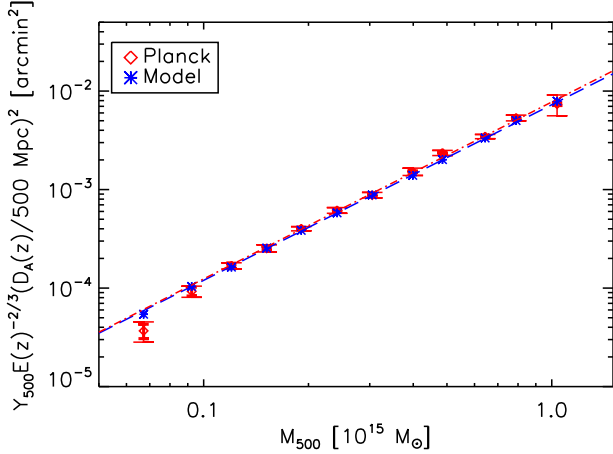
Fig. 5. Scaling relation between Planck SZ signal and total mass. Symbols and lines are as in Fig. 4.
