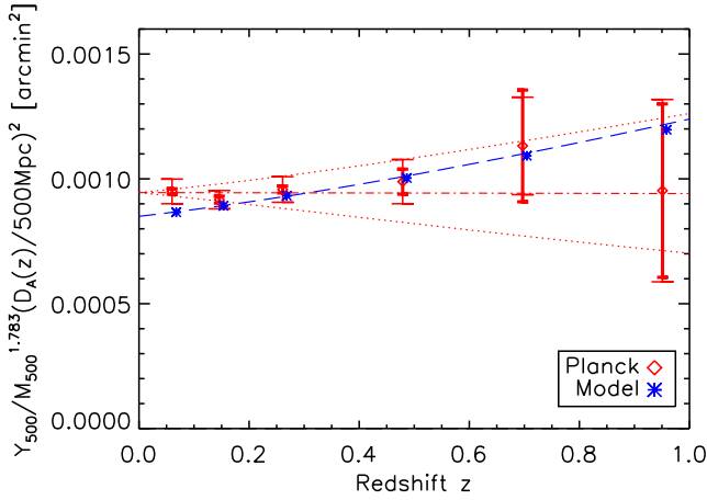
Fig. 6. Bin averaged SZ signal from a sphere of radius R_{500} ( Y_{500} ) scaled by the expected mass and angular distance dependence as a function of redshift. The Planck data (red diamonds) and the SZ cluster signal expected from the X-ray based model (blue stars) are shown together with the expected standard redshift evolution (dashed line). The best fitting model is shown by the dot-dashed line and the 1\sigma confidence region is limited by the dotted lines. Here M_{500} is given in units of 3 \times 10^{14} M_{\odot} .
