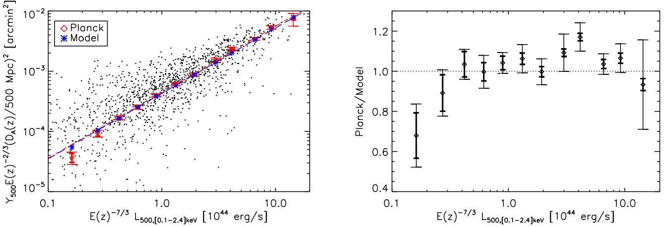
Fig. 4. Left: Scaling relation between Planck SZ measurements and X-ray luminosity for \sim 1600 MCXC clusters. Both quantities are intrinsic and scaled assuming standard evolution. Individual measurements are shown by the black dots and the corresponding bin averaged values by the red diamonds. Thick bars give the statistical errors, while the thin bars are bootstrap uncertainties. The bin-averaged SZ cluster signal expected from the X-ray based model is shown by the blue stars. The combination of the adopted D_A^2 Y_{500} - M_{500} and L_{500} - M_{500} relations (Eq. 6) is shown by the dashed blue line while the red dot-dashed line shows the best fitting power-law to the data (Eq. 7 and Table 4). Right: Ratio between data and model bin averaged values shown in the left panel. Error bars are as in the left panel.
