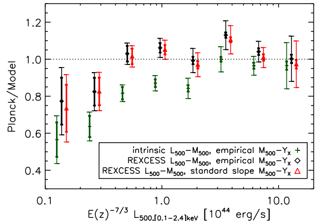
Fig. 9. Ratio of binned Planck data points to model for different model assumptions. The fiducial model (black diamonds) is shown together with results obtained by varying the underlying L_{500} - M_{500} relation from REXCESS to intrinsic (green plus signs), and by varying the slope of the underlying M_{500} - Y_X relation from empirical to standard (red triangles). Thick bars give the statistical errors, while the thin bars are bootstrap uncertainties.
