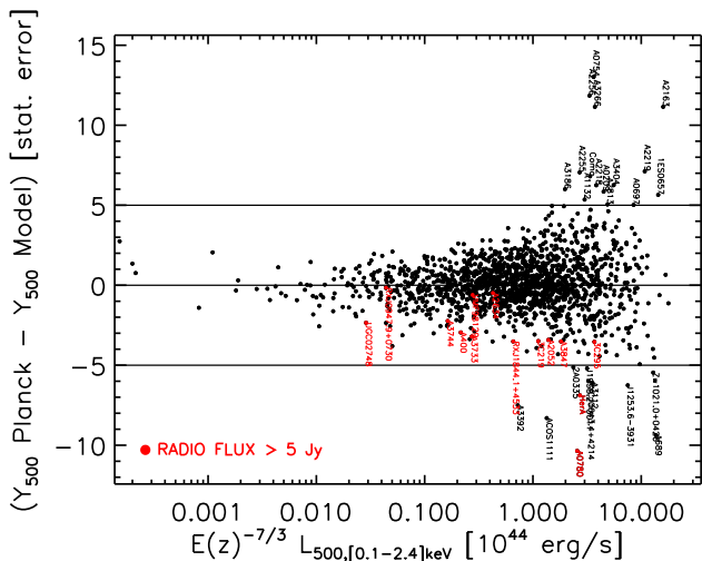
Fig. 8. Difference between the Planck measurement and the X-ray based prediction in units of the measurement statistical error (pure measurement uncertainties based on MMF noise estimates) as a function of X-ray luminosity. Outliers at more than 5\sigma , which are discussed in the text, are labelled by their name. Clusters with SZ signal possibly contaminated by radio sources (see discussion in Sect. 6) are shown in red and labelled by their name.
