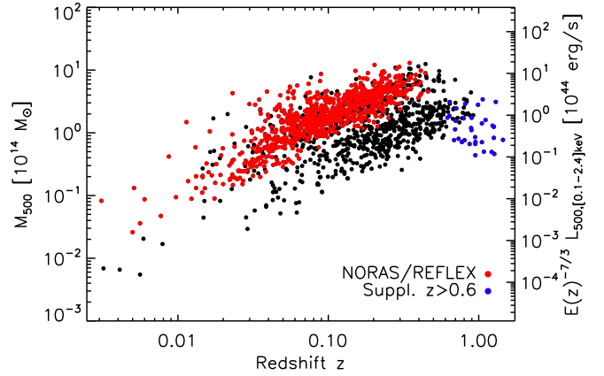
Fig. 1. Observed [0.1-2.4] keV band luminosities (right vertical axis) and inferred masses (left vertical axis) as a function of redshift. Shown are the MCXC (the NORAS/REFLEX control sub-sample is shown in red) and the supplementary clusters (blue dots).
