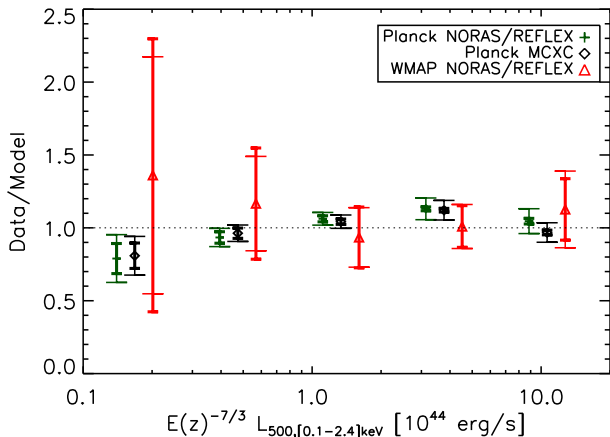
Fig. 10. Data-to-model ratio for Planck results for the full sample (black diamonds) and the NORAS/REFLEX control sample (green plus signs). The WMAP -5yr results for the NORAS/REFLEX by Melin et al. (2010) are shown by the red triangles. Error bars are as in Fig. 4.
