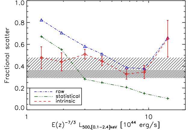
Fig. 7. Fractional raw (dot-dashed blue line and triangles), statistical (dot-dot-dashed green line and plus signs), and intrinsic (dashed red line, diamonds, and error bars) scatter on the D_A^2 Y_{500} - L_{500} relation. The coarse/fine-hatched regions corresponds to the 1\sigma uncertainties on the intrinsic scatter reported in Arnaud et al. (2010) and Planck Collaboration (2011g), respectively.
