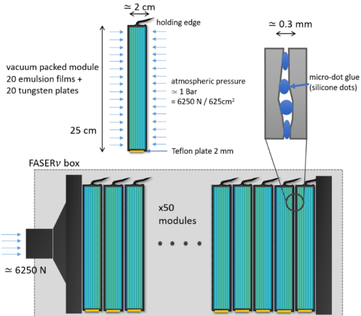
Vacuum-packed module
