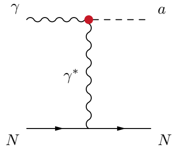
ALP production via the Primakoff process from photons scattering in the TAN
