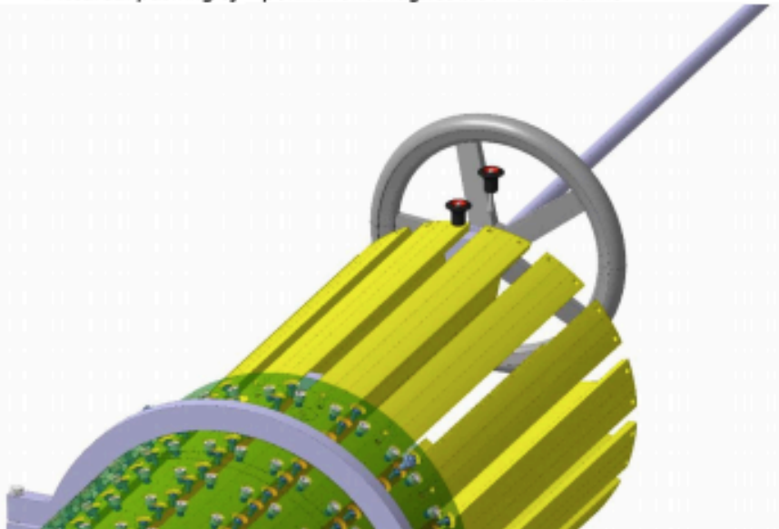
Pictured: pushing of 1 permanent magnet block at the time
