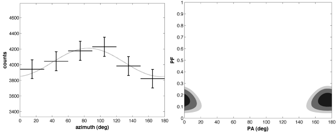
FIG. 1.—Azimuthal profile, modulation angle, PA, and fraction, PF = a_0/a_{100} , measured for a sample of unpolarized spurious events obtained during the Crab observations. The error bars for the profile are at 1\sigma . The 68%, 95%, and 99% confidence regions are shaded from dark to light gray.
