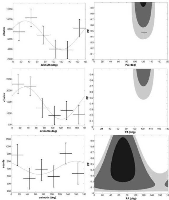
FIG. 2.—Azimuthal profile, modulation angle, PA, and fraction, PF = a_{\phi}/a_{100} , measured for the Crab data between 200 and 800 keV, in the off-pulse (top), off-pulse and bridge (middle), and two-peak (bottom) phase intervals. The error bars for the profile are at 1\sigma . The 68%, 95%, and 99% confidence regions are shaded from dark to light gray. The SPI result (Dean et al. 2008) is indicated in the top figure by a cross.
